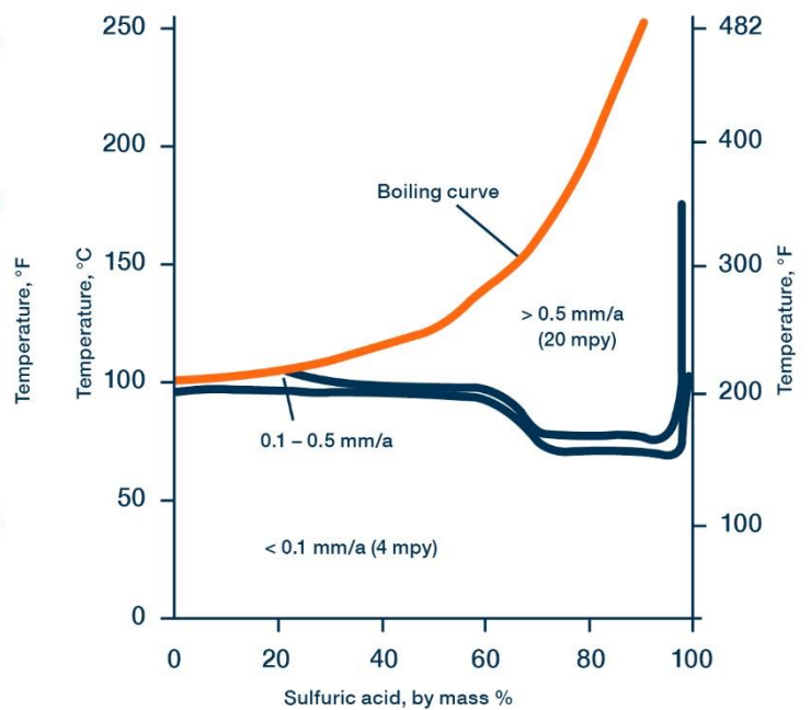
Fig. 2: ISO corrosion diagram of VDM® Alloy 59 in sulfuric acid, as calculated based on static immersion tests over at least 120h
